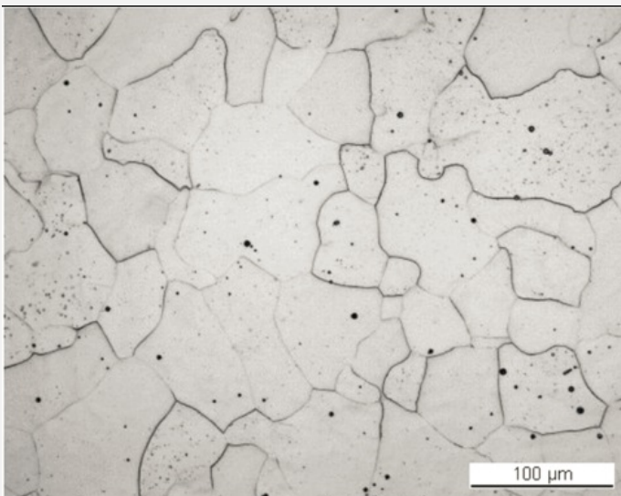
Fig. 6: Micrograph of the metal sample from Fig. 3 (detail), nital etched, bright field. The metal presents a ferritic structure,
