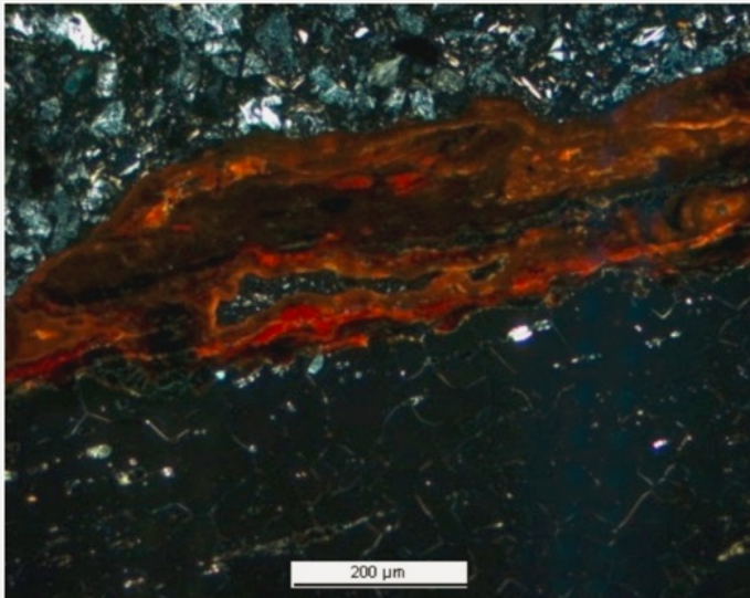
Fig. 11: Micrograph (same as Fig. 10) unetched, polarised light. We observe from bottom to top: a red-orange inner corrosion layer, followed by a dark-brown intermediate layer and an orange-brown outer layer,
