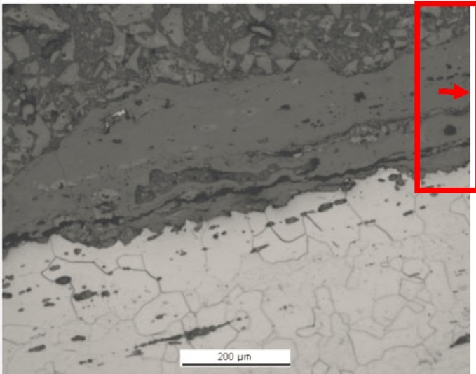
Fig. 10: Micrograph showing the metal - corrosion layer interface from Fig. 3 (reversed picture, detail), unetched, bright field. The grey corrosion layer contains bright inclusion rows. The rectangle marks one part of the mapped area in Fig. 12,
