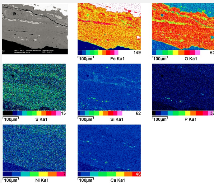
Fig. 12: SEM image, BSD-mode, and elemental chemical distribution of the selected area from Fig. 10 (inversed, detail). Method of examination: SEM/EDX, Laboratory of Analytical Chemistry, Empa,
