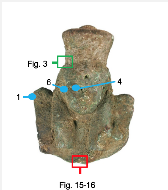
Fig. 2: Front face: location of XRF measurements (blue spots), powder sample (red square) and gilding remains on the surface (green square),
