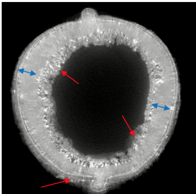
Fig. 11: X-ray tomography by cross section of the crown shows a dense and non-porous metal core (blue arrows). The corrosion products however are porous (red arrows). The external limitos is visible as a fine line preserved under corrosion layers,
