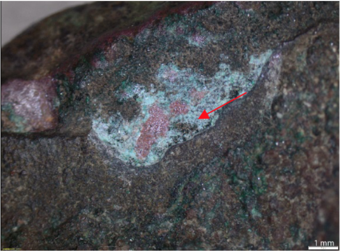
Fig. 15: Observation of the light green corrosion product,
