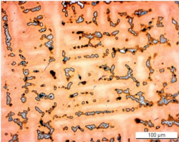
Fig. 6: Micrograph of the metal sample from Fig. 3 (detail), etched, bright field. The leaded bronze has the dendritic structure of an as-cast metal with the Sn-rich eutectoid alpha + delta phase appearing in white at the dendrites borders,
