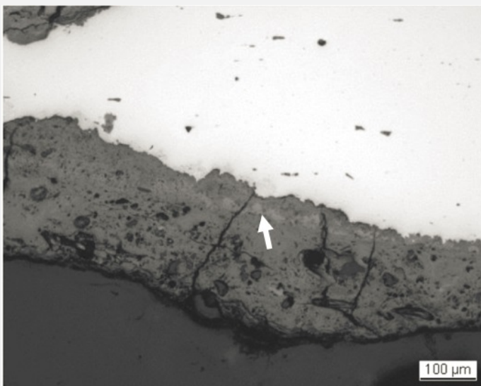
Fig. 11: Micrograph showing the metal - corrosion crust interface from Fig. 3 (detail of Fig. 12), unetched, bright field. The heterogeneous and heavily cracked corrosion layer appears grey enclosing a light-grey layer (indicated by an arrow),
