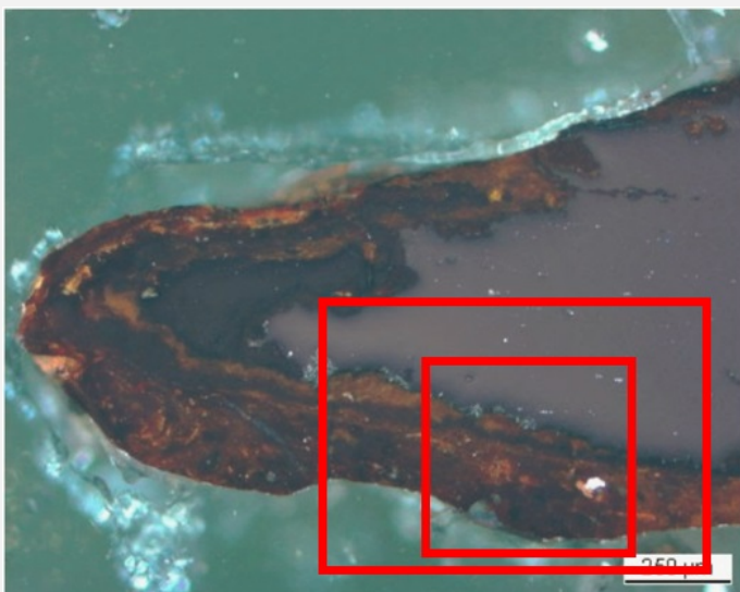
Fig. 12: Micrograph showing the metal - corrosion crust interface from Fig. 3 (detail) unetched, polarised light. The micrographs of Fig. 11 and Fig. 13 are marked by the large and small rectangles respectively. The light-grey layer of Fig. 11 (arrow) appears black whereas the rest of the corrosion layer is brown, red and orange,
