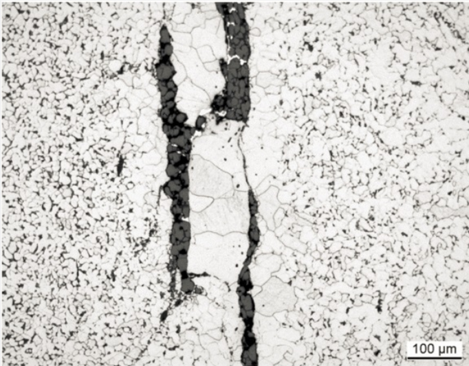
Fig. 9: Micrograph of cross-section from Fig. 3 (detail), nital etched, bright field. We observe a hypoeutectoid steel including a ferritic zone surrounded by slag inclusions,
