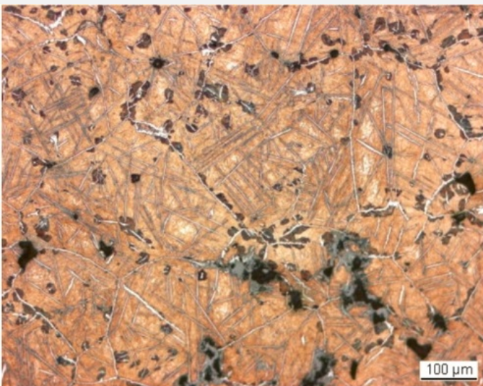
Fig. 9: Micrograph of the metal sample, detail from Fig. 5, etched, bright field. Hypereutectoid steel with a structure of cementite in white in the grain boundaries and in needle form combined with martensite (pink). Some bainite occurs around the grain boundaries,
