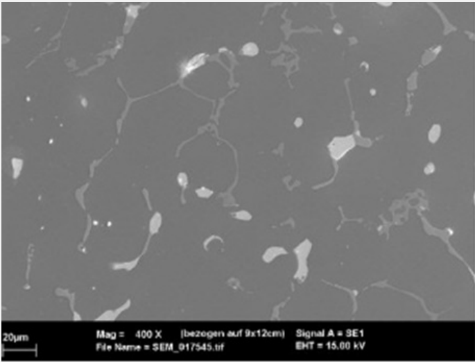
Fig. 6: SEM image of the metal sample from Fig. 3 (detail), SE-mode, unetched. We observe in dark-grey the metal matrix, in medium-grey the intermetallic compound Al 2 Cu as well as Al, Fe, Si & Cu phase clusters and in light-grey the Sn inclusions,
