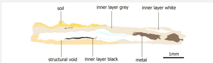
Fig. 16: Improved stratigraphic representation of the stratigraphy of corrosion layers on the military tag from visual observations and analyses,
