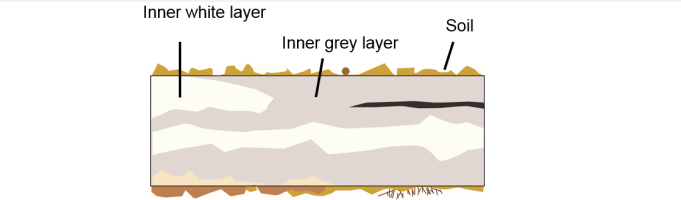
Fig. 3: Stratigraphic representation of the military tag in cross-section by macroscopic observation,
