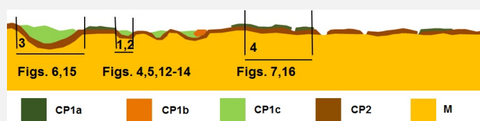
Fig. 9: Location of the samples on the stratigraphic representation of Fig. 8,
