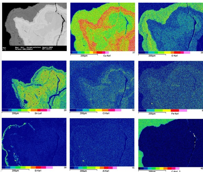
Fig. 9: SEM image, BSE-mode, and elemental chemical distribution of the selected area from Fig. 3 (reversed picture, detail). Method of examination: SEM/EDS, Laboratory of Analytical Chemistry, Empa,
