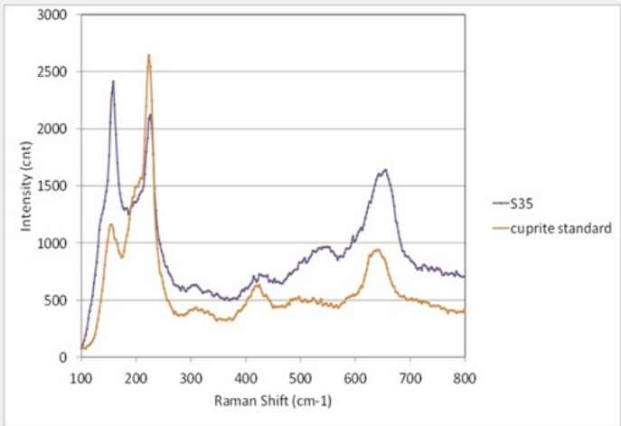
Fig. 10: Raman spectrum of CP3 (S35) from Fig. 8 compared to a cuprite standard spectrum. Settings: laser wavelength 532nm, acquisition time 20s, one accumulation, filter D2 (0.75-0.8mW), hole 1000, slit 100, grating 600. Method of analysis: Raman spectroscopy, Lab of Swiss National Museum, Affoltern a. Albis ZH,
