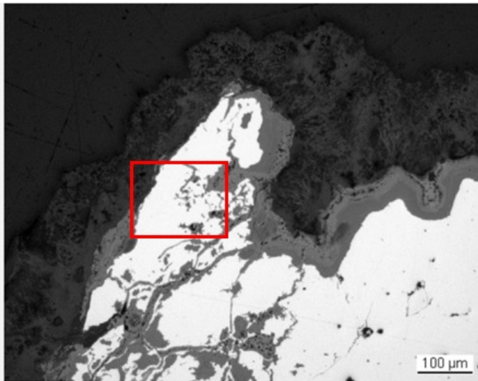
Fig. 5: Micrograph of the metal sample from Fig. 3 (detail), unetched, bright field. From bottom right to top left we observe: the metal (in white) with porosity (in black) and the corrosion layer (in light and dark-grey). The micrograph of Fig. 6 is marked by a rectangle,
