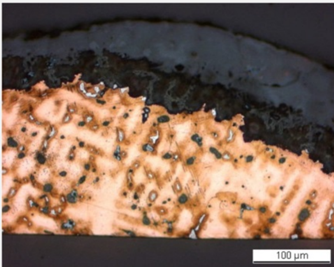
Fig. 6: Micrograph similar to Fig. 5, etched, bright field. The dendritic structure of the leaded bronze is revealed with the alpha-delta eutectoid in white and the alpha phase in pink. The colour difference of the alpha phase is due to coring,
