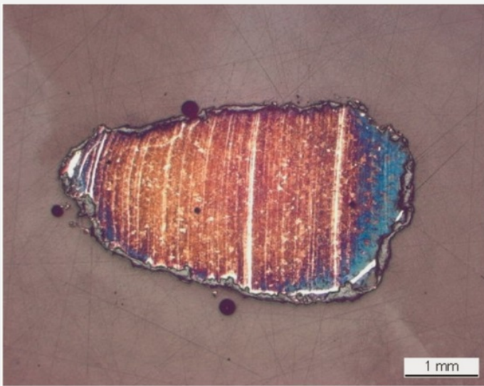
Fig. 6: Micrograph of the metal sample from Fig. 3, etched with Oberhoffer's reagent, bright field. We observe three P-rich welding seams in white,
