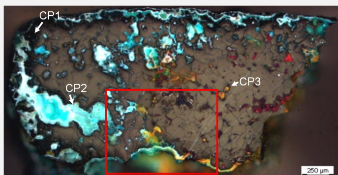
Fig. 7: Micrograph of the cross-section (same as Fig. 3) and corresponding to the stratigraphy of Fig. 4, polarised light, showing the location of Fig. 8,
