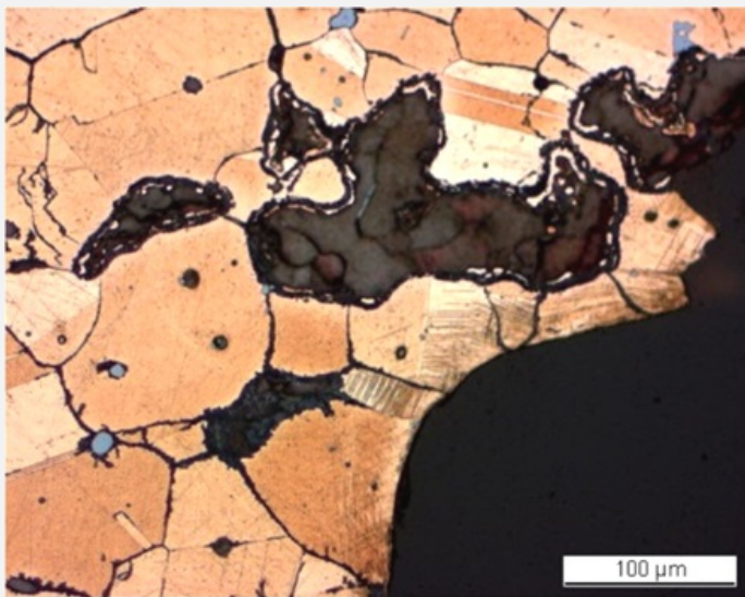
Fig. 6: Micrograph of the metal sample from Fig. 3 (detail), etched, bright field. We observe pink-orange polygonal grains with twins and slip lines as well as copper sulphide inclusions (in blue),
