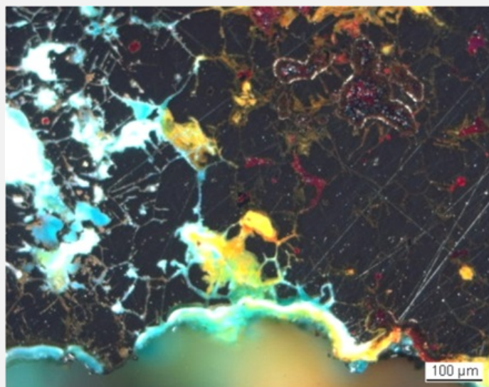
Fig. 8: Micrograph (same as Fig. 5), polarised light. In black the metal. Blue-green, orange and red corrosion products are found in the porous metal and along the grain boundaries,
