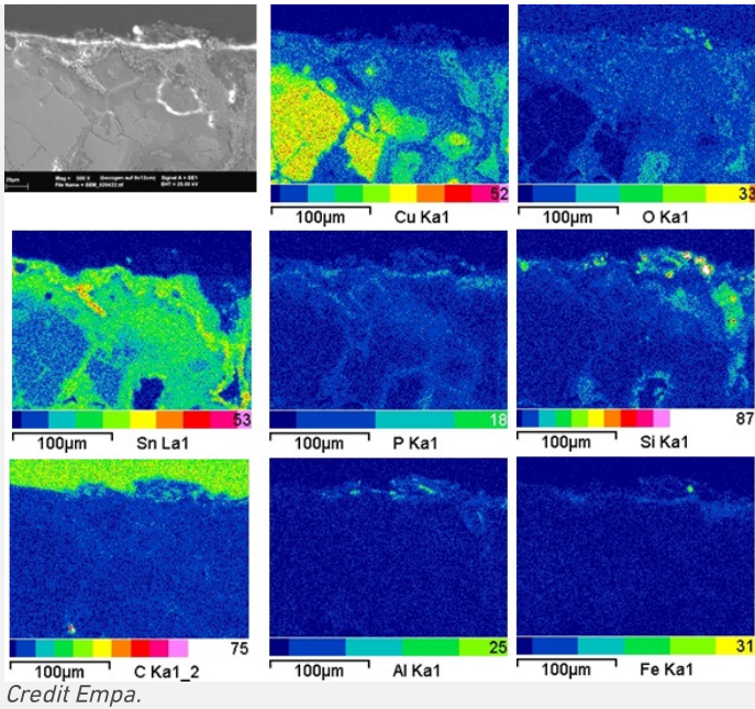
Fig. 9: SEM image, SE-mode, and elemental chemical distribution of the selected area from Fig. 3. Method of examination: SEM/EDS, Laboratory of Analytical Chemistry, Empa,
