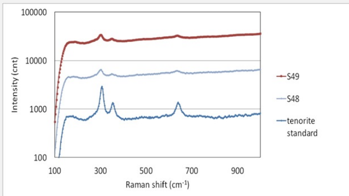
Fig. 10: Raman spectra of the outer dark corrosion layer (S48 and S49) compared to a tenorite standard spectrum. Settings: laser wavelength 532nm, acquisition time 20s for S48 and 100s for S49, one accumulation, filter D1 (7.5-8mW), hole 500, slit 80, grating 600. Method of analysis: Raman spectroscopy, Lab of Swiss National Museum, Affoltern a. Albis ZH,
