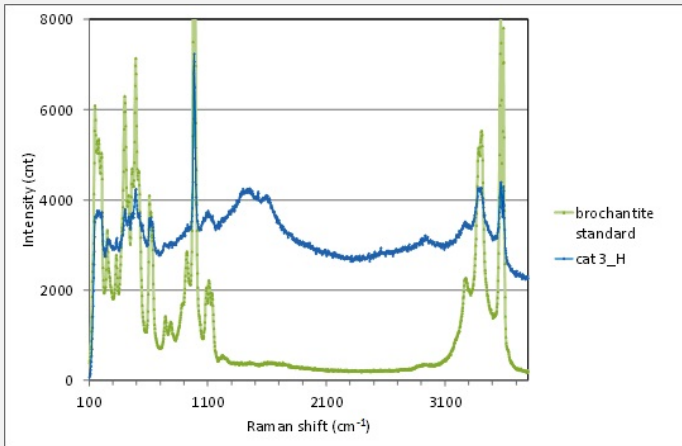
Fig. 10: Raman spectrum of the green outer corrosion layer (CP1) of the external side (cat3_H) compared to a brochantite standard spectrum. Settings: laser wavelength 532nm, acquisition time 100s, one accumulation, filter D2 (0.75-0.8 mW), hole 500, slit 80, grating 600. The peak indicated with an arrow on the cat3_H spectrum is due to fluorescence. Method of analysis: Raman spectroscopy, Lab Swiss National Museum, Affoltern a. Albis ZH,
