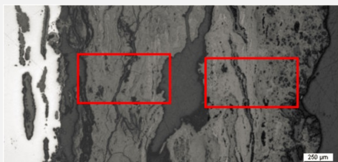
Fig. 11: Micrograph showing the metal - corrosion crust interface from Fig. 3 (reversed picture, detail), unetched, bright field. The micrographs of Fig. 13 (left) and Fig. 14 (right) are marked by rectangles,
