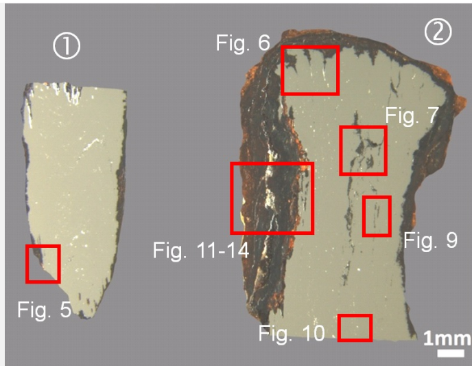
Fig. 3: Micrograph of the cross-sections from samples 1 and 2 showing the location of Figs. 5 to 7 and 9 to 14,
