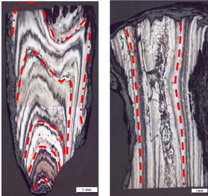
Fig. 8: Micrograph of metal samples 1 and 2, etched with Oberhoffer's reagent, bright field. The P segregation along the welding seams is outlined. The main welding seams are marked by red dotted lines,
