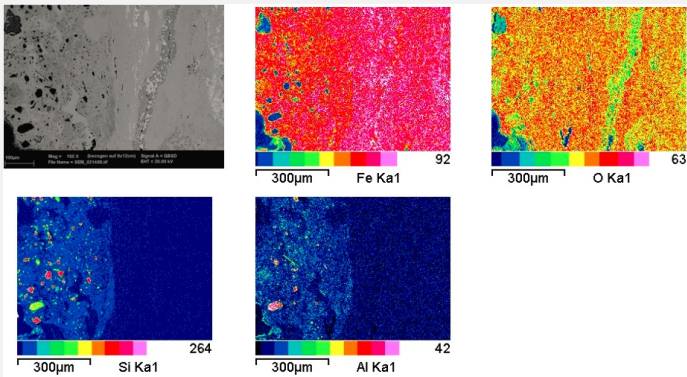
Fig. 14: SEM image, BSE-mode, and elemental chemical distribution of the selected area from Fig. 10 (reversed picture). Method of examination: SEM/EDS, Laboratory of Analytical Chemistry, Empa,
