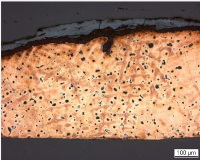
Fig. 6: Micrograph of the metal sample from Fig. 3 (detail), etched, bright field. The dendritic structure is revealed with dark-grey lead inclusions and porosities (in black),
