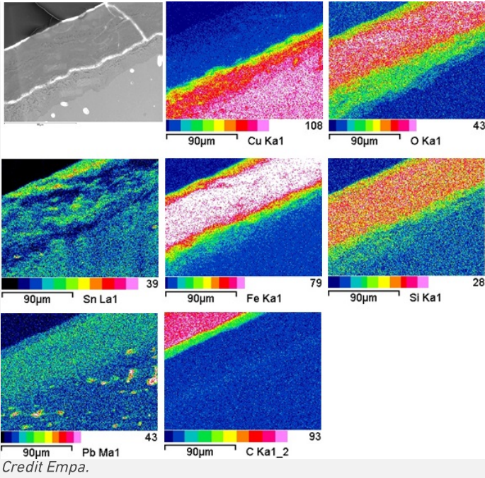
Fig. 9: SEM image, SE-mode, and elemental chemical distribution of a selected area of Fig. 7. The Pb mapping includes the Pb and copper sulphide inclusions, because of a peak interference. Method of examination: SEM/EDS, Laboratory of Analytical Chemistry, Empa,
