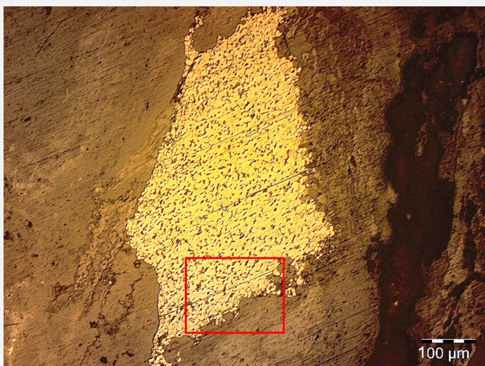
Fig. 9: Micrograph of the metal sample from Fig. 7 (detail, rotated 90 degrees), Nital etched, bright field,
