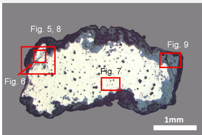
Fig. 3: Micrograph of the cross-section showing the location of Figs. 5 to 9,
