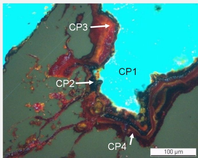
Fig. 8: Micrograph showing the metal - corrosion crust interface from Fig. 3 (detail of Fig. 5) and corresponding to the stratigraphy of Fig. 4, polarised light. From bottom left to to right: In grey the metal, in dark-red/orange CP4, in light red CP3, in black (with pores) CP2 and in green-blue CP1,
