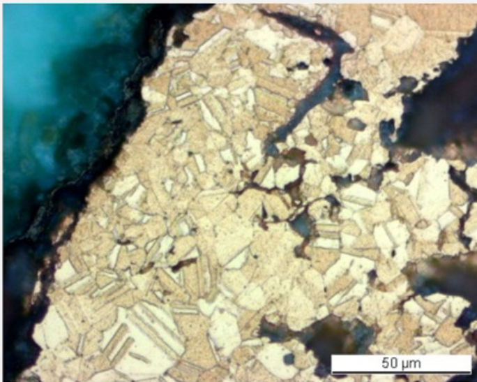
Fig. 6: Micrograph of the metal sample from Fig. 3 (detail of Fig. 5), etched, bright field. The metal shows a structure of mostly small polygonal grains with twins,
