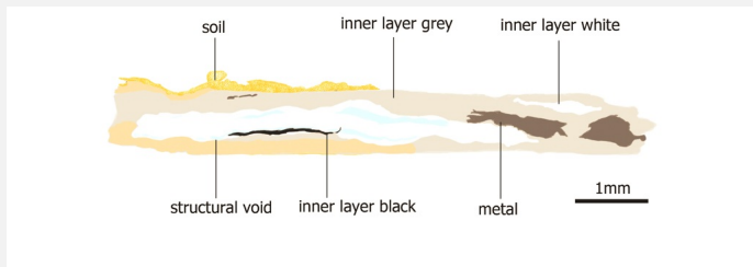
Fig. 16: Improved stratigraphic representation of the stratigraphy of corrosion layers on the military tag from visual observations and analyses,
