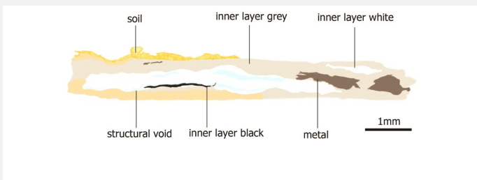
Fig. 16: Improved stratigraphic representation of the stratigraphy of corrosion layers on the military tag from visual observations and analyses,
