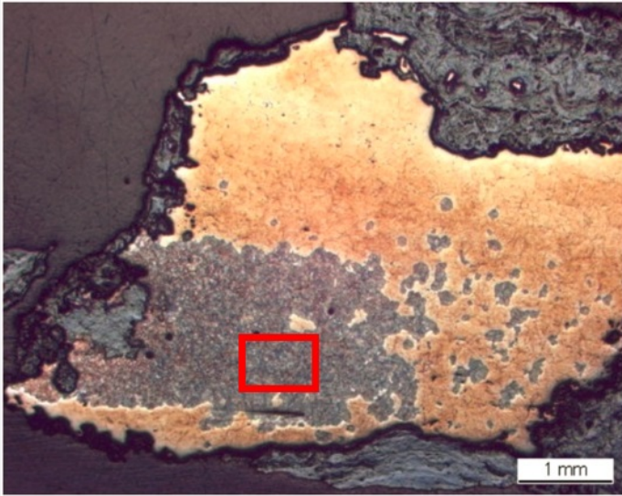
Fig. 7: Micrograph of the metal sample from Fig. 3 (inverted picture, detail), etched, bright field. We observe the metal with martensite (orange) and bainite nodules (blue). The micrograph of Fig. 10 is marked by a rectangle,
