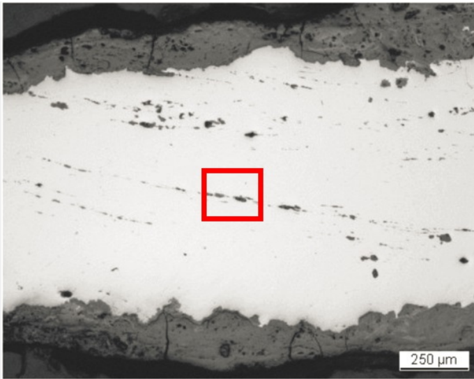
Fig. 5: Micrograph of the metal sample from Fig. 3 (detail), unetched, bright field. In white the metal, in light-grey the slag inclusions and the corrosion layer. The micrograph of Fig. 6 is marked by a rectangle,
