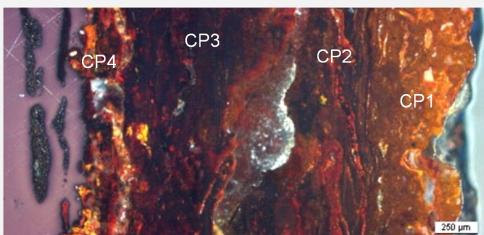
Fig. 12: Micrograph (same as Fig. 11) corresponding to the stratigraphy of Fig. 4, unetched, polarised light. From left to right: the metal in violet, the successive corrosion layers having a yellow (CP4), grey (CP3) to dark-red colour (CP2). The outer layer is orange-brown with quartz inclusions in white (CP1),
