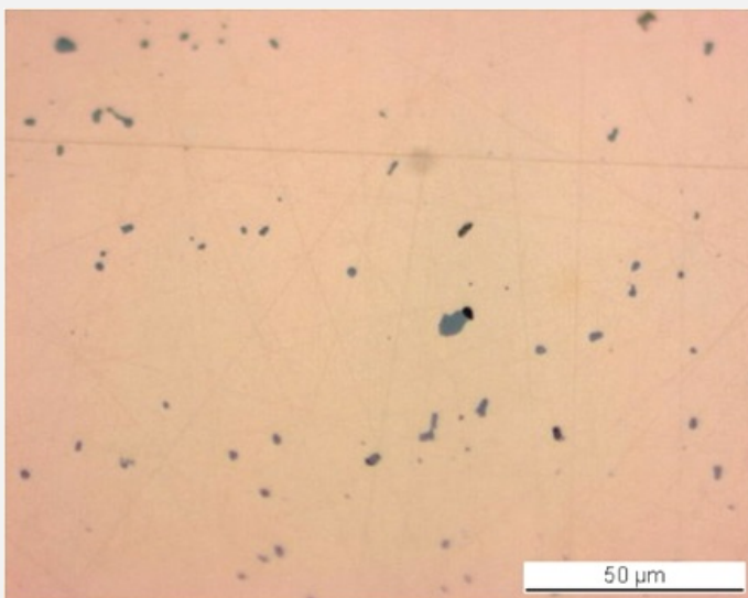
Fig. 5: Micrograph of the metal sample from Fig. 3 (detail), unetched, bright field. Grey copper sulphide inclusions are clearly visible,
