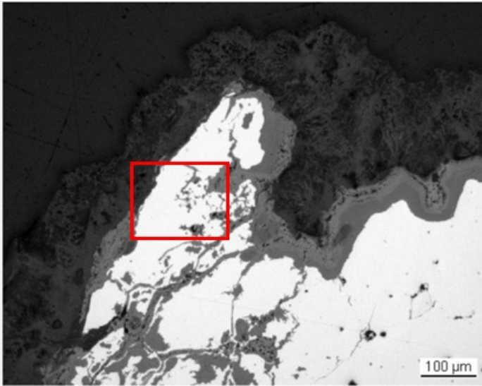
Fig. 5: Micrograph of the metal sample from Fig. 3 (detail), unetched, bright field. From bottom right to top left we observe: the metal (in white) with porosity (in black) and the corrosion layer (in light and dark-grey). The micrograph of Fig. 6 is marked by a rectangle,
