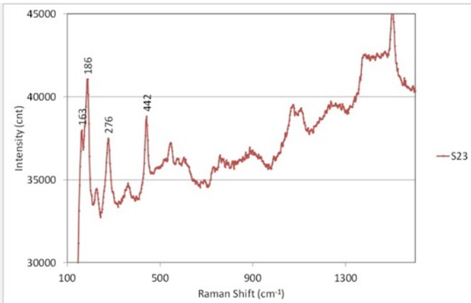
Fig. 12: Raman spectrum of the green outer corrosion layer (CP1) from Fig. 8. Settings: laser wavelength 532nm, acquisition time 80s, one accumulation, filter D2 (0.75-0.8mW), hole 500, slit 80, grating 600. Method of analysis: Raman spectroscopy, Lab of Swiss National Museum, Affoltern a. Albis ZH,
