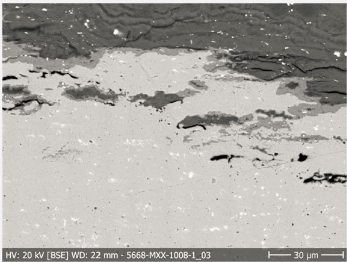
Fig. 8: SEM image of the cross-section, from Fig. 5 (detail), BSE-mode,
