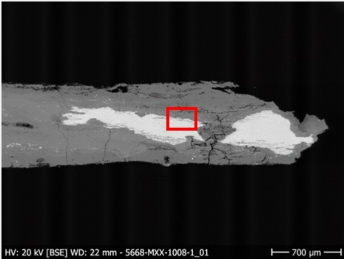
Fig. 7: SEM image of the cross-section, from Fig. 4 (detail), BSE-mode. Note the presence of Pb inclusions all through the thickness of the heavily cracked corrosion layers,
