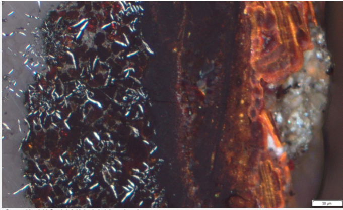
Fig. 11: Micrograph similar to Fig. 10 but under polarized light. The external deposit (D1) appears grey-white, CP1 in bright orange, while CP2 and CP3 appear dark red to brown. The corroded metal (CM1) contains remnants of graphite flakes (in white) and the P-rich eutectic (in grey),
