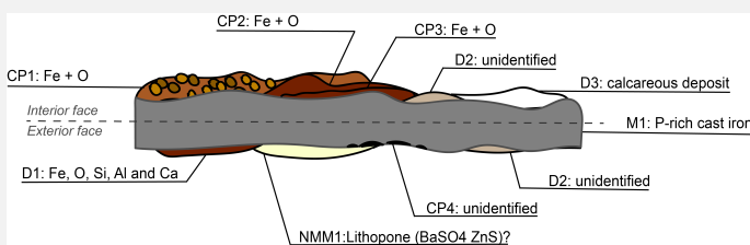
Fig. 13: Improved stratigraphic representation of the rain gutter fragment with results of SEM-EDS analysis and visual microscopic observation,
