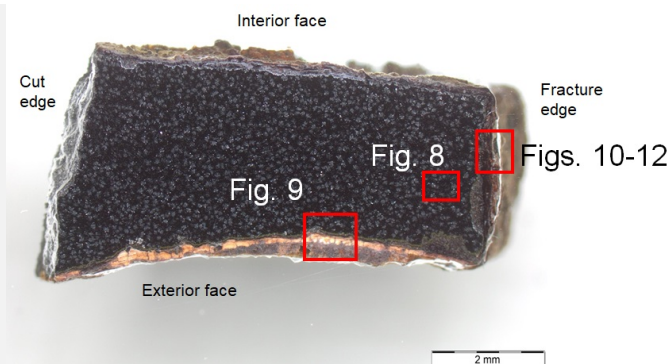
Fig. 4: Micrograph of the sample taken from the rain gutter fragment showing its orientation relative to the artefact and the locations of Figs. 8-12,
