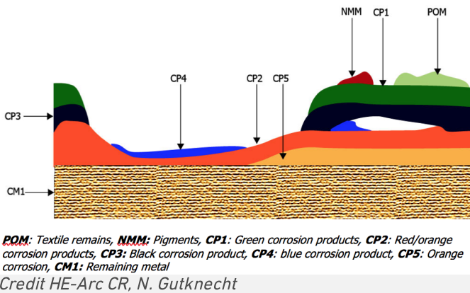
Fig. 3b: Stratigraphic representation of the back face of the funeral mask in cross-section by macroscopic observation,
