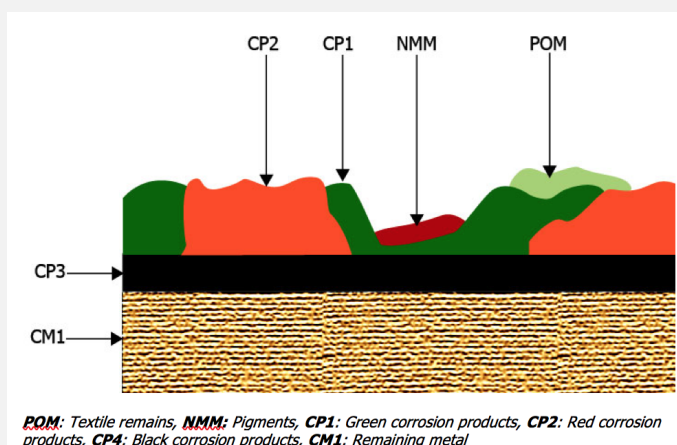
Fig. 3a: Stratigraphic representation of the front face of the funeral mask in cross-section by macroscopic observation,
