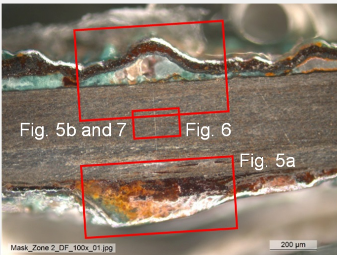
Fig. 4: Micrograph of the cross-section of the sample temporarily taken from the detached fragment of Fig. 2 showing the locations of Figs. 5a (corresponding to the front of the funeral mask), Fig. 5b (back of the funeral mask), Figs. 6 and 7,
