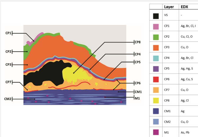
Fig. 16: Improved stratigraphic representation of the funeral mask (Fig. 7) based on the results from the SEM-EDS analyses,
