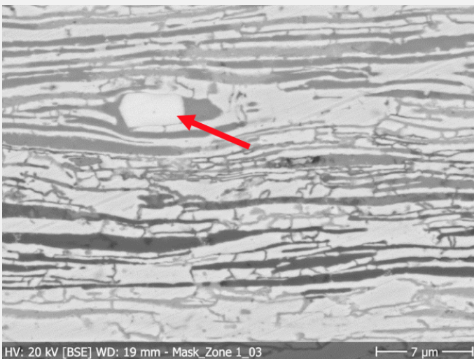
Fig. 6: SEM image (BSE-mode) of the metal sample from Fig. 4 (detail), the elongated grains are the result of repeated hammering. Absence of strain lines indicates that the metal is annealed. The darker areas are Cu-rich phases and the lighter areas are Ag-rich phases. The arrow shows an As- and Pb inclusion,
