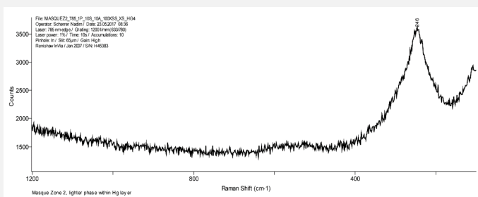
Fig. 15: Raman analysis of the mercury compounds from the cross section. Method of analysis: Raman spectroscopy, HKB,
