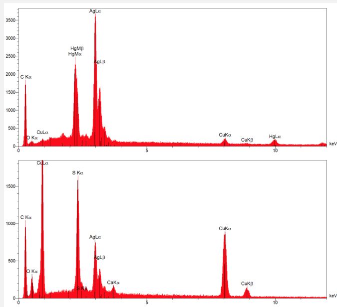
Figs. 11 a and b: EDS analysis of the layer that appears light grey under polarized light, situated below the red layer (Fig. 4). Method of analysis: SEM-EDS, Lab of Electronic Microscopy and Microanalysis, IMA (Néode), HEI Arc,
