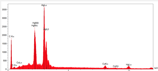
Figs. 11 a and b: EDS analysis of the layer that appears light grey under polarized light, situated below the red layer (Fig. 4). Method of analysis: SEM-EDS, Lab of Electronic Microscopy and Microanalysis, IMA (Néode), HEI Arc,
