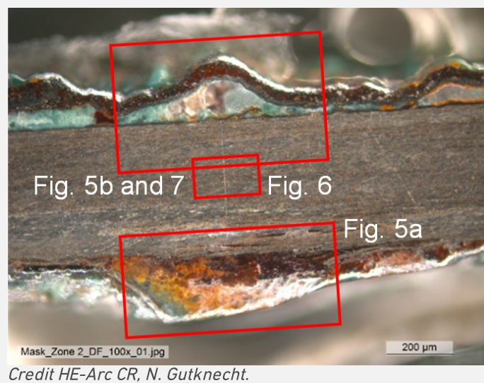
Fig. 4: Micrograph of the cross-section of the sample temporarily taken from the detached fragment of Fig. 2 showing the locations of Figs. 5a (corresponding to the front of the funeral mask), Fig. 5b (back of the funeral mask), Figs. 6 and 7,
