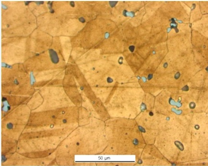
Fig. 6: Micrograph of the metal sample from Fig. 3 (detail), etched, bright field. Angular and twinned grains are revealed as well as copper sulphide inclusions in grey,
