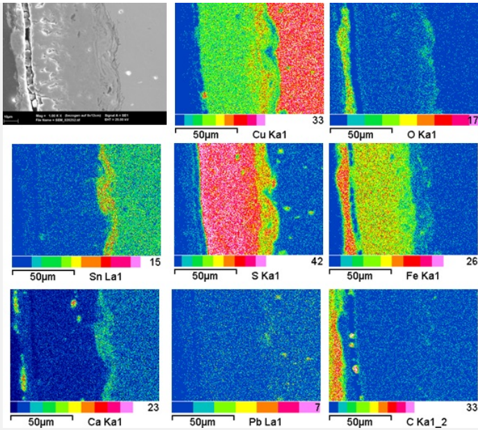
Fig. 10: SEM image, SE-mode, and elemental chemical distribution of the selected area of Fig. 7 (reversed picture). Method of examination: SEM/EDS, Laboratory of Analytical Chemistry, Empa,
