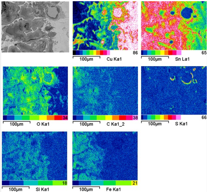
Fig. 10: SEM image, SE-mode, and elemental chemical distribution of the selected area of Fig. 7 (reversed picture rotated by 270°). Method of examination: SEM/EDS, Laboratory of Analytical Chemistry, Empa,
