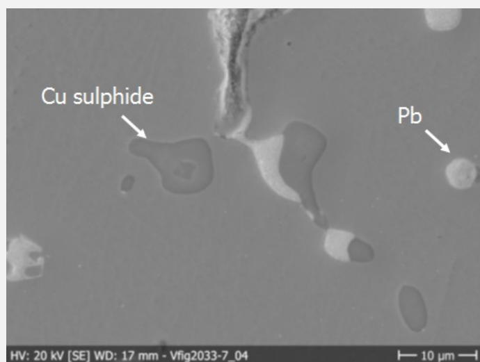
Fig. 7: SEM image (detail of Fig. 6), SE-mode, showing copper sulphide and lead inclusions,
