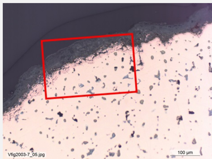
Fig. 6: Micrograph of the cross-section of sample from Fig. 2 of the headrest (or horse bit) (detail of Fig. 4), unetched, bright field. Light grey copper sulphide and tiny round Pb inclusions as well as "porosities" can be observed. Area of Fig. 10 is marked by a red rectangle,
