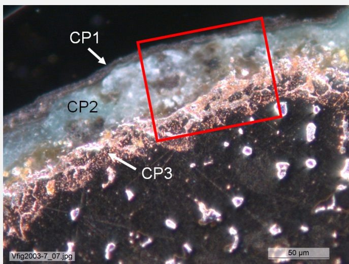
Fig. 11: Micrograph similar to Fig. 10 and corresponding to the stratigraphy of Fig. 5, polarised light. The area selected for elemental chemical distribution (Fig. 12) is marked by a red rectangle,
