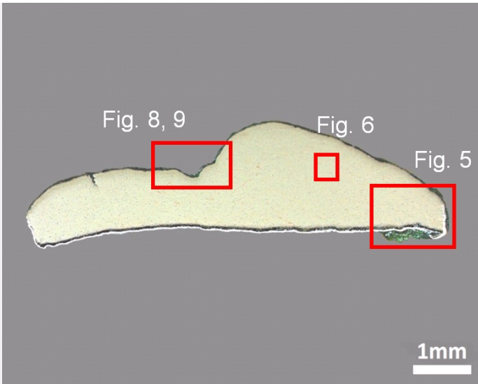
Fig. 3: Micrograph of the cross-section of the sample taken from the circular base showing the location of Figs. 5 to 6 and 8 to 9,
