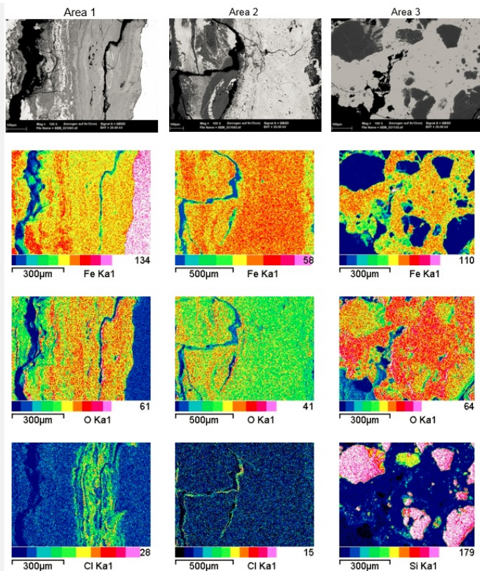
Fig. 9: SEM images, BSE-mode, and elemental chemical distribution of the selected areas from Figs. 7 and 8 (reversed picture rotated by 270°, details). First column: mapping on area 1 (CP3) where an inner layer enriched in Cl appears near the metal surface. 2nd column: area 2 (CP2) where iron oxides prevail. 3rd column: area 3 (CP1) where the outer O-rich layer includes rock fragments rich in Si. Method of examination: SEM/EDS, Lab. Anal. Chem. Empa,
