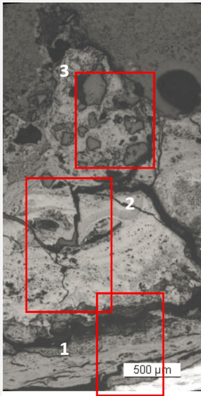
Fig. 7: Micrograph of the corrosion layer from Fig. 3 showing the metal - corrosion crust interface (detail, rotated by 45°) and corresponding to the stratigraphy of Fig. 4, unetched, bright field. The areas 1 (for CP3), 2 (for CP2) and 3 (for CP3) selected for elemental chemical distribution (Fig. 9) are marked by red rectangles,
