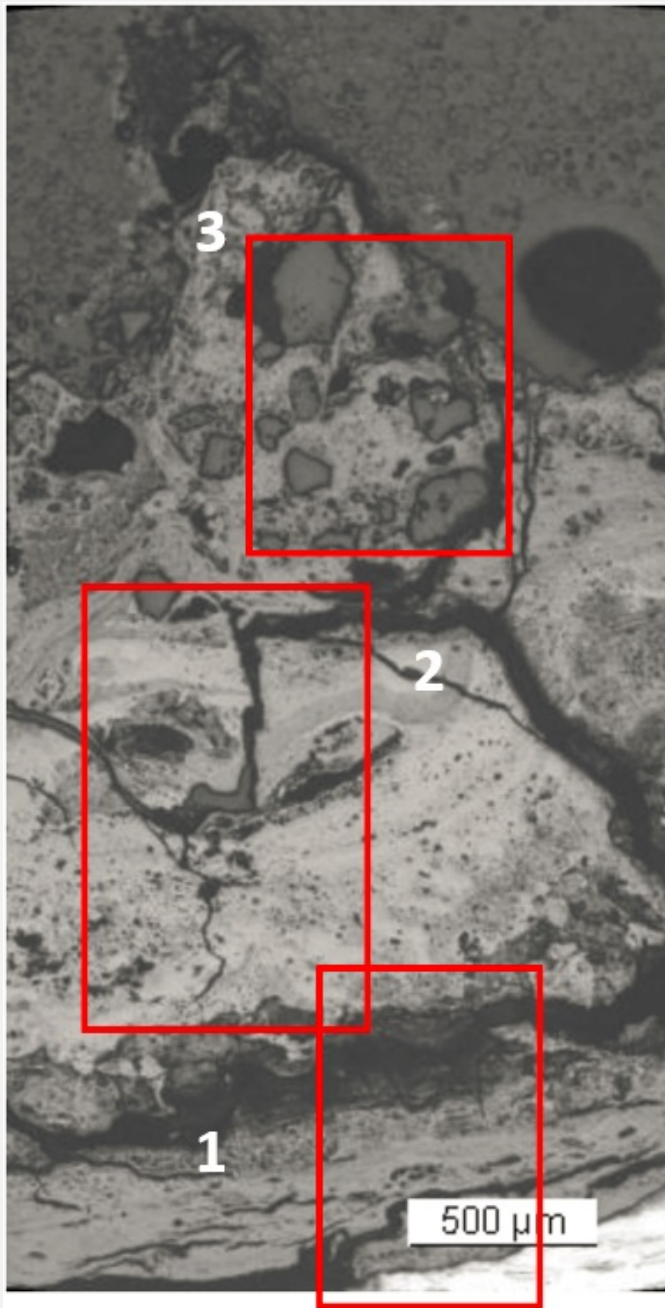
Fig. 7: Micrograph of the corrosion layer from Fig. 3 showing the metal - corrosion crust interface (detail, rotated by 45°) and corresponding to the stratigraphy of Fig. 4, unetched, bright field. The areas 1 (for CP3), 2 (for CP2) and 3 (for CP3) selected for elemental chemical distribution (Fig. 9) are marked by red rectangles,
