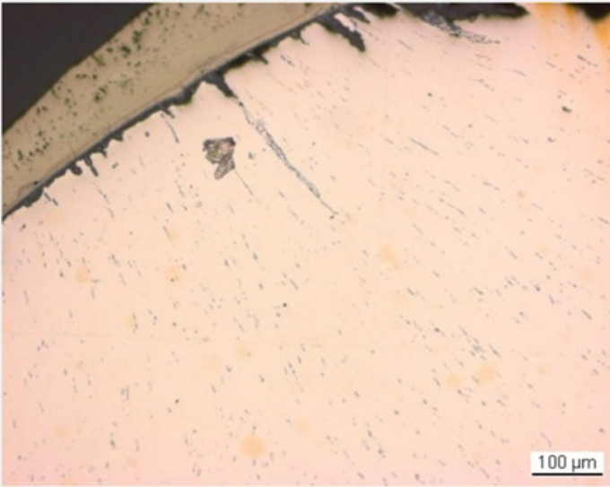
Fig. 5: Micrograph of the metal sample from Fig. 3 (detail), unetched, bright field. Rows of elongated copper sulphide inclusions can be observed,
