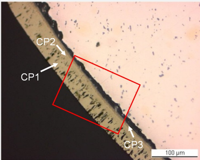
Fig. 10: Micrograph of the metal sample from Fig. 3 (detail) and corresponding to the stratigraphy of Fig. 4, unetched, bright field. The area selected for elemental chemical distribution (Fig. 12) is marked by a red rectangle,
