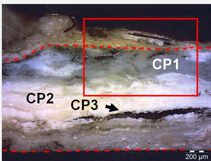
Fig. 10: Micrograph of the cross-section, from Fig. 4 (detail) and corresponding to the stratigraphy of Fig. 5, unetched, dark field, 50x. View of the inner layers and the limit of the original surface (red line). We can see that the interfaces between the different layers are not well defined: some of the white corrosion product is found inside the inner grey layer. The micrograph of Fig. 11 is marked by a rectangle,
