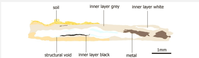
Fig. 16: Improved representation of the stratigraphy of corrosion layers of the military tag from visual observations and analyses,
