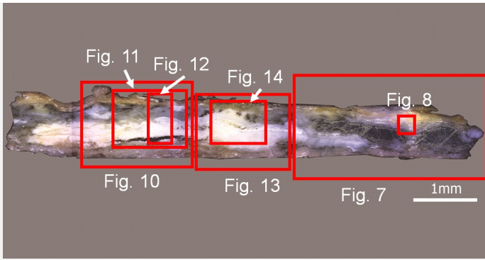
Fig. 4: Micrograph of the cross-section of fragment b of the military tag showing the location of Figs. 7, 8 and 10 to 14. Unetched, dark field, 50x,
