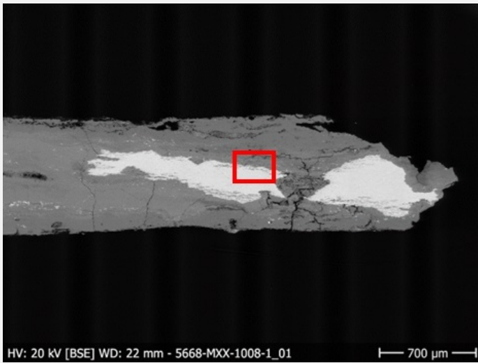
Fig. 7: SEM image of the cross-section, from Fig. 4 (detail), BSE-mode. Note the presence of Pb inclusions all through the thickness of the heavily cracked corrosion layers. The SEM image of Fig. 8 is marked by a rectangle,
