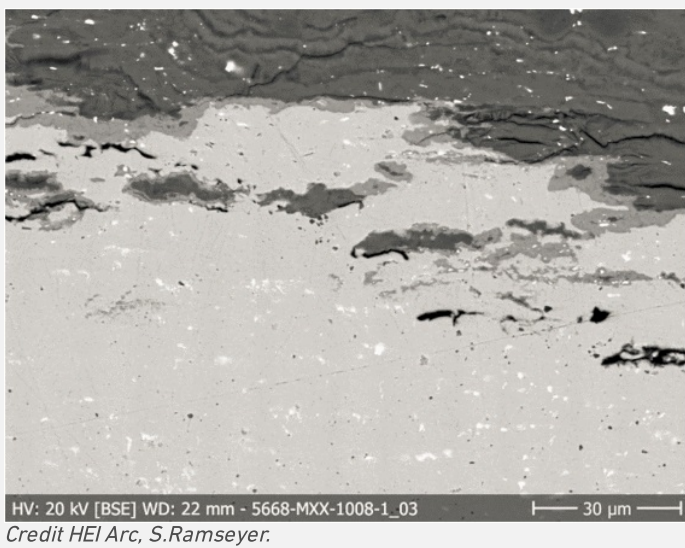
Fig. 8: SEM image of the cross-section, from Fig. 7 (detail), BSE-mode,
