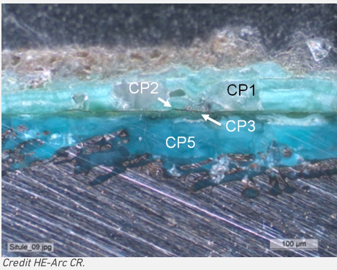
Fig. 13: Micrograph of the metal / corrosion interface (detail of Fig. 10) unetched, dark field, 100x. The outer layer (CP1 of Fig. 6) incorporates soil material and the thin dark layer (CP2 of Fig. 6) highlights the limit of the original surface,
