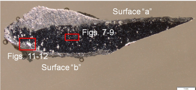
Fig. 4: Micrograph of the sample taken from the roof gutter showing the locations of Figs. 7-9 and 11-12. The uppermost area (in white) is remains of solder, while the zinc metal appears dark grey to black (the white patches are due to secondary oxidation of the sample),
