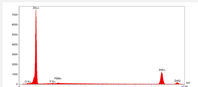
Fig. 6: Chemical composition of the metal. Method of analysis: SEM-EDS. Lab. of Electronic Microscopy and Microanalysis, Néode, HEI Arc,
