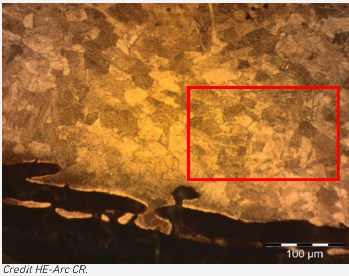
Fig. 8: Micrograph of the metal structure from Fig. 7 (detail), etched, bright field, 50x. The alpha phase of the alloy shows polygonal grains. Area of Fig. 9 is marked by a red rectangle,
