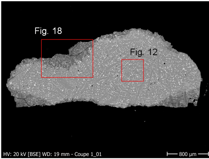
Fig. 11: SEM image of the cross-section similar to Fig. 8, BSE-mode. The area selected for elemental chemical analysis (Fig. 12) is marked by a rectangle. Fig. 18 is similarly indicated.
