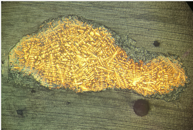
Fig. 13 : Micrograph showing the dendritic microstructure (reversed picture of Fig. 11), etched, bright field.
