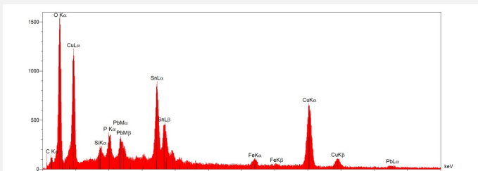
Fig. 20: EDS spectrum of the area (CP1) located in Fig. 18.
