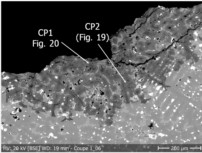
Fig. 18: SEM picture showing interdendritic corrosion with locations of Figs. 19 and 20.
