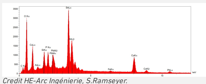
Fig. 19: EDS spectrum of the area (CP2) located in Fig. 18.
