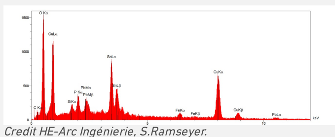
Fig. 20: EDS spectrum of the area (CP1) located in Fig. 18.
