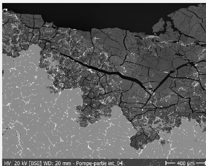
Fig. 12: SEM image (BSE mode) of the selected area (in blue) of the sample shown on Fig. 7, showing the remaining metal on the bottom and CM1 /CPs on top,
