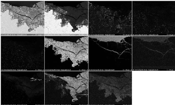
Fig. 15: SEM image and elemental chemical distribution of the area of Fig. 12. Method of analysis: SEM-EDS. Lab. of Electronic Microscopy and Microanalysis, Néode, HEI Arc,
