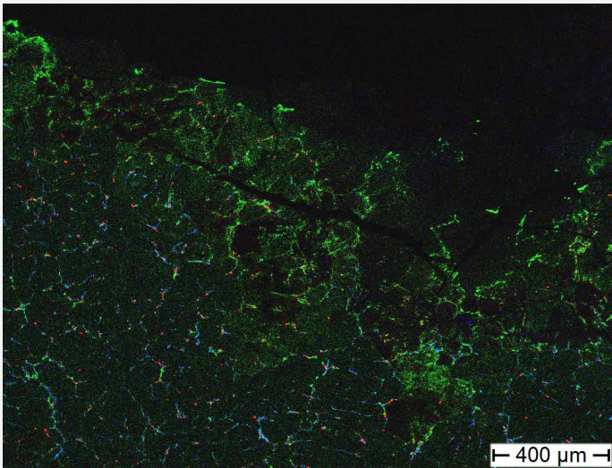
Fig. 14: Sn (red), Fe (blue) and Cu (green) distribution of the area of Fig. 12. Method of analysis: SEM-EDS. Lab. of Electronic Microscopy and Microanalysis, Néode, HEI Arc,
