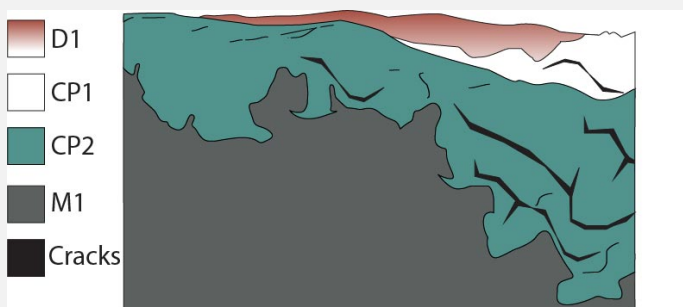
Fig. 6: Stratigraphic representation of the corroded exit pipe of the water pump in cross-section by macroscopic observation, M = metal, CP = corrosion product, D = deposit,
