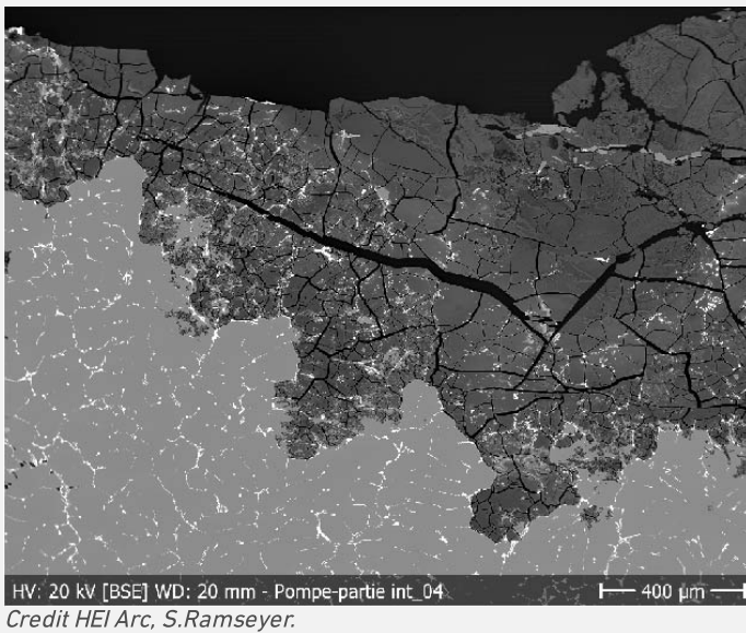
Fig. 12: SEM image (BSE mode) of the selected area (in blue) of the sample shown on Fig. 7, showing the remaining metal on the bottom and CM1 /CPs on top,
