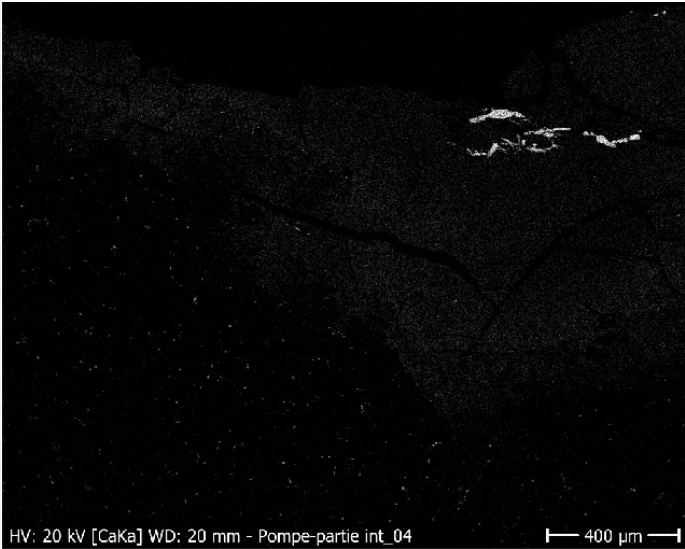
Fig. 16: Ca distribution of the area of Fig. 12. Method of analysis: SEM-EDS. Lab. of Electronic Microscopy and Microanalysis, Néode, HEI Arc,
