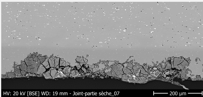
Fig. 12: SEM image (BSE mode) of the cross-section of zone 2 of the gasket (detail of Fig. 8) showing the core metal on top (M2) and the heavily corroded colaminated metal (M1),
