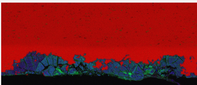
Fig. 13: Al (red), O (blue) and Fe (green) chemical distribution of the area of Fig. 12. Method of analysis: SEM-EDS. Lab. of Electronic Microscopy and Microanalysis, Néode, HEI Arc.
