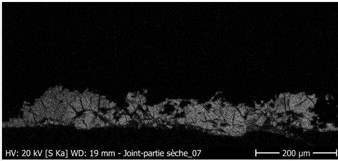
Fig. 14: S chemical distribution of the area of Fig. 12. Method of analysis: SEM-EDS. Lab. of Electronic Microscopy and Microanalysis, Néode, HEI Arc.
