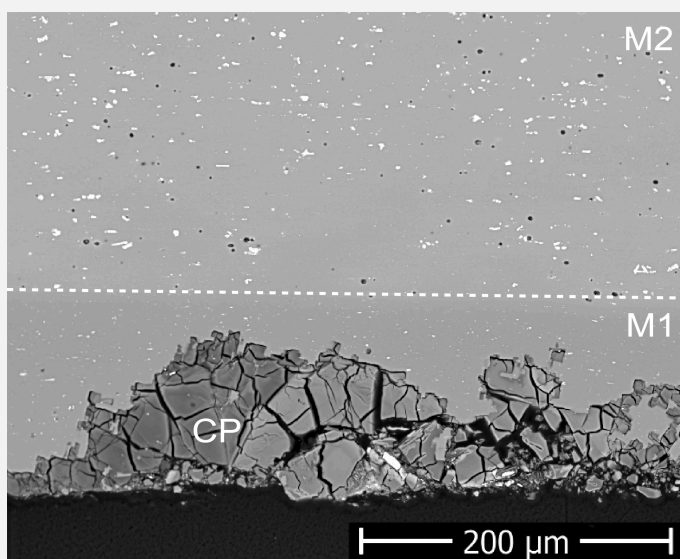
Fig 9: SEM detail (BSE mode) of zone 1 of the colaminated sheet in cross-section. The core metal (M2) is porous (in black) and shows oriented inclusions (in white) and the colaminated metal (M1) is compact and has smaller oriented inclusions (in white). Corrosion products (in dark grey) are limited to M1,
