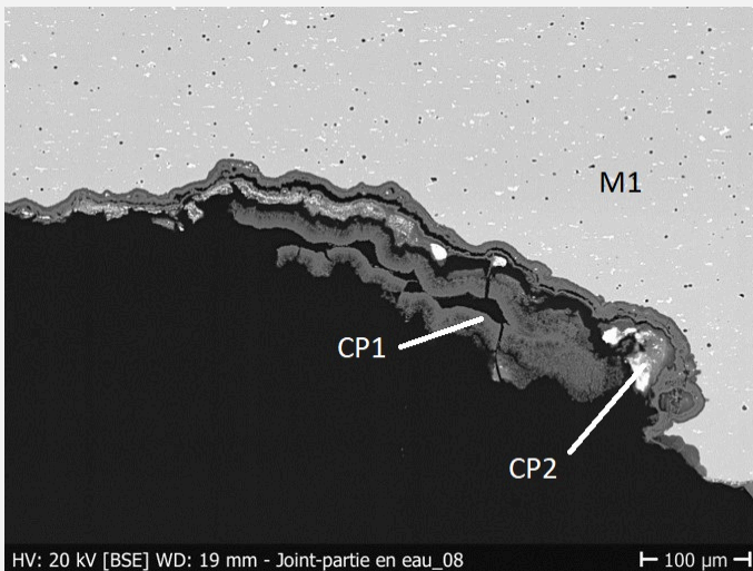
Fig 11: SEM detail (BSE mode) of zone 1 of the gasket in cross-section. The colaminated Al is missing. The core metal (now M1) is porous (black spots) and shows oriented inclusions (in white). The corrosion products (CP1) are very friable and retain clusters of inclusions that are also corroded (CP2),
