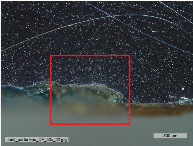
Fig. 10: Micrograph of the cross-section of the gasket, zone 2, shown on Fig. 5 unetched, dark field, showing the location of the SEM image of Fig. 11 (in red),
