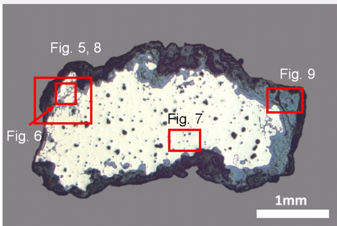
Fig. 3: Micrograph, in bright field, of the cross-section of the sample taken from the bed structure showing the location of Figs. 5 to 9,
