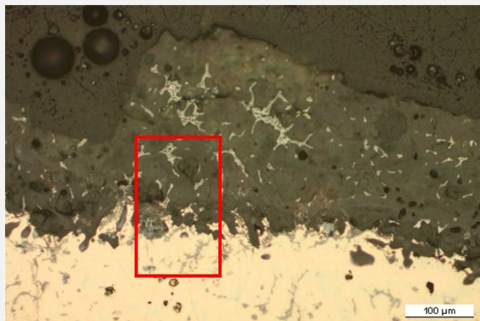
Fig. 7: Micrograph of the metal sample from Fig. 3 (rotated 180°), unetched, bright field. A metallic ghost structure is preserved in the corrosion crust. The area selected for elemental chemical distribution (Fig. 10) is marked by a red rectangle,
