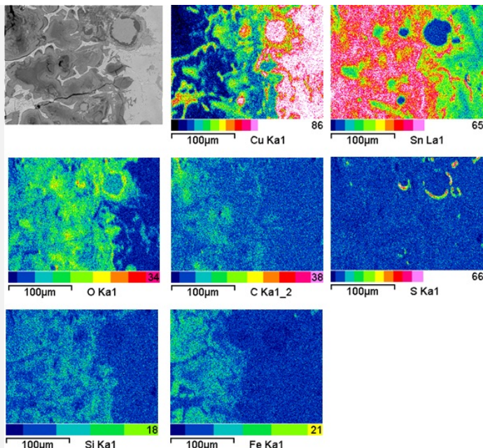
Fig. 10: SEM image, SE-mode, and elemental chemical distribution of the selected area of Fig. 7 (reversed picture rotated by 270°). Method of examination: SEM/EDS, Laboratory of Analytical Chemistry, Empa,
