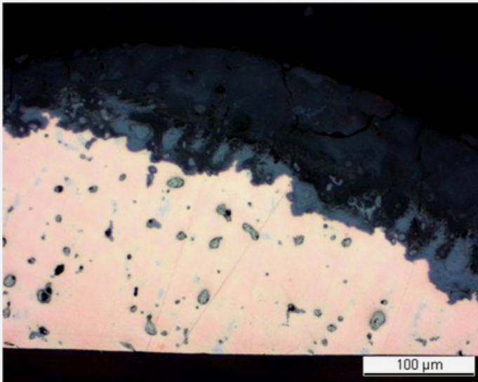
Fig. 5: Micrograph of the metal sample from Fig. 3 (detail), unetched, bright field. The metal is in pink, the Pb-rich inclusions in light-grey, the copper sulphide inclusions in dark-grey and the alpha-delta eutectoid in light-blue,
