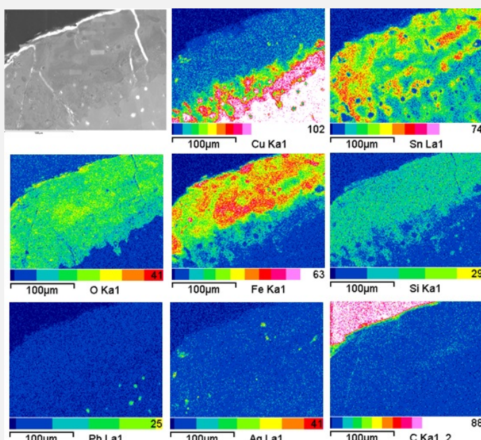
Fig. 8: EDS elemental chemical distribution in an SEM image (detail of Fig. 5, reversed picture). Method of examination: SEM/EDS, Laboratory of Analytical Chemistry, Empa,
