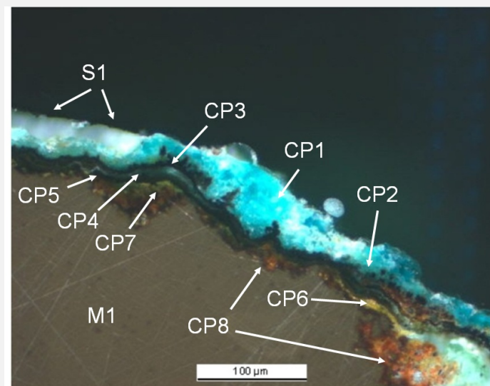
Fig. 9: Micrograph of the metal sample from Fig. 4 and corresponding to the stratigraphy of Fig. 5, polarised light. The metal appears in brown; the inner layer appears as red-orange, the intermediate layer as black and the outer layer as turquoise,
