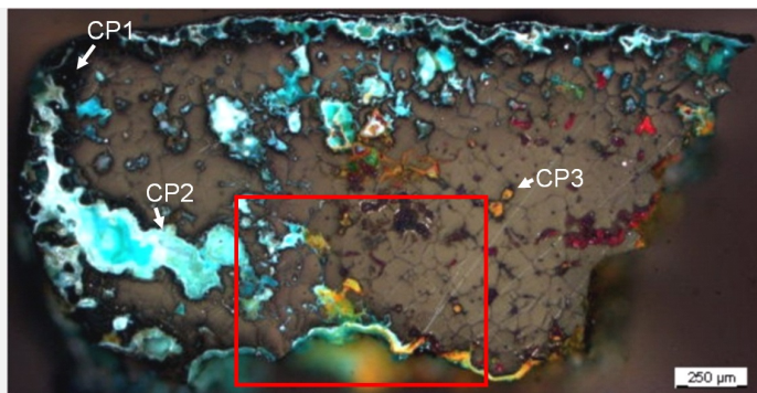
Fig. 7: Micrograph of the cross-section of the metal sample (same as Fig. 3) and corresponding to the stratigraphy of Fig. 4, polarised light, showing the location of Fig. 8,
