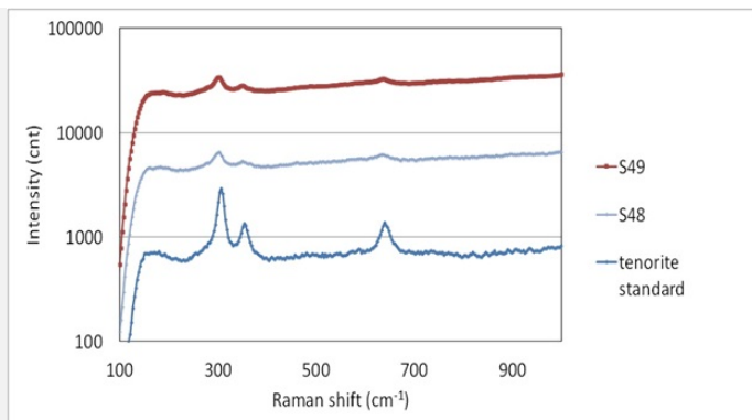
Fig. 10: Raman spectra of the outer dark corrosion layer (S48 and S49) compared to a tenorite standard spectrum. Settings: laser wavelength 532nm, acquisition time 20s for S48 and 100s for S49, one accumulation, filter D1 (7.5-8mW), hole 500, slit 80, grating 600. Method of analysis: Raman spectroscopy, Lab of Swiss National Museum, Affoltern a. Albis ZH,
